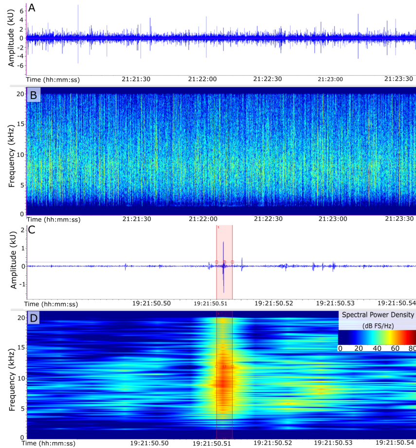
Figure 4.3: SoundTrap 500 recordings were bandpass-filtered (1.5-20 kHz), visualized in Raven Pro as A a full-spectrum waveform with RMS amplitude (blue) and B spectrogram, plotting intensity (dB FS/Hz) normalized to 1 Hz bandwidth. C Example waveform amplitude (blue line) identifying single snap exceeding the 1000 U threshold (shaded in red); D spectrogram from the same time (snap shaded in red).
