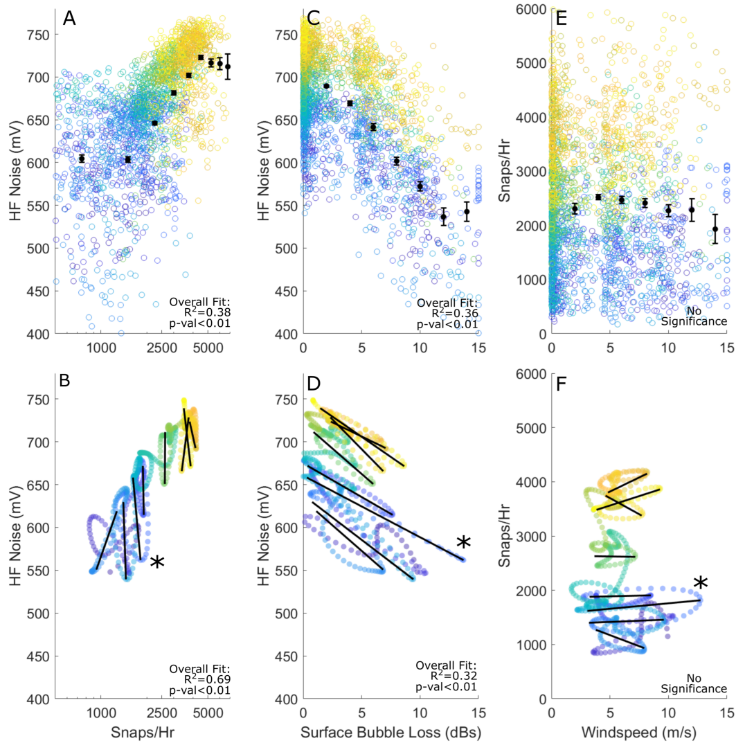
Figure 4.10: Hourly averages from spring ( n=2268 hrs) of A raw and B filtered snap rate and HF noise (mV), on a log scale; C raw and D filtered SBL (dB) and HF noise (mV); E raw and F filtered snap rate and wind speed (m/s). Marker color represents the date range, January (blue) to May (yellow). Reported statistics include all plotted data; "no significance" represents p\text{-values}>0.01 . Binned averages are shown over the raw data (black markers) in A , C , E , and significant wind events are denoted (black lines) in B , D , F . See Figure 4.11 for a closer examination of an isolated wind event (*).
