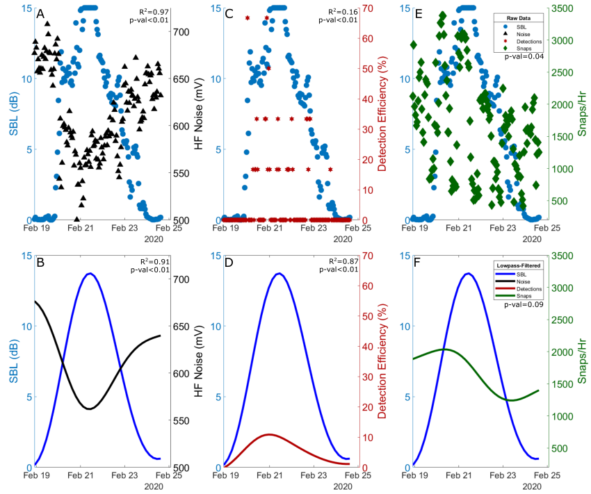
Figure 4.11: Example of a single wind event, Feb. 19th-25th 2020, with 0.3-14.3 m/s wind speed. A Raw and B low pass SBL (dB) and HF noise (mV), C raw and D low pass SBL (dB) and detections, and E raw and F low pass SBL (dB) and snap rate.
