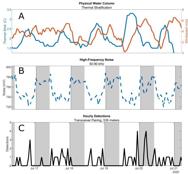
Figure 3.6: Time series of A bulk thermal stratification and wind magnitude, B high-frequency noise from SURTASSTN20, and C isolated detections from STSNew1 to SURTASSTN20, two VR 2 Tx transceivers that were 535 meters apart. Night is shaded in B and C .
