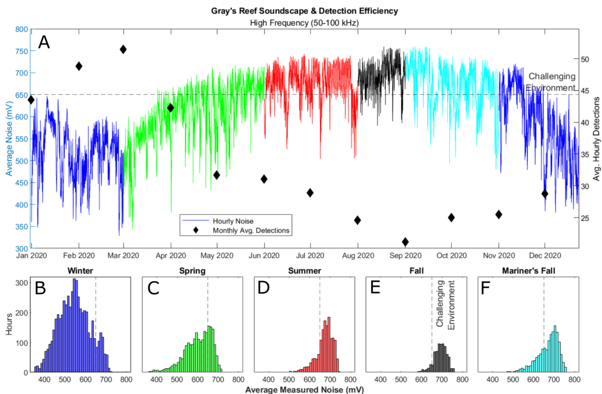
Figure 3.3: Time series of high frequency noise from SURTASS05IN at Gray's Reef colored by season: winter (blue), spring (green), summer (red), fall (black), and mariner's fall (teal). A Hourly HF noise (line) compared to the average hourly detections (diamonds) collected that month, with (–) denoting a challenging acoustic environment. B-F histograms of hourly average noise for each season.
